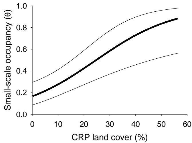
Figure 7. The small-scale occupancy rate, probability of occupancy of 7.5\text{-km} \times 7.5\text{-km} quadrants by lesser prairie-chickens given occupancy of the 15\text{-km} \times 15\text{-km} grid cells, plotted as a function of Conservation Reserve Program (CRP) land cover for the shortgrass habitat region of northwest Kansas. The bold line was the model-averaged estimate of small-scale occupancy from using the models in Table 6. The bounding lines were unconditional 95% confidence intervals.
