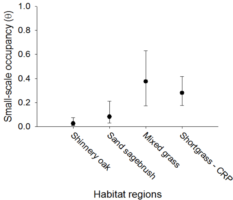
Figure 8. The small-scale occupancy rate, probability of occupancy in 7.5\text{-km} \times 7.5\text{-km} quadrats by lesser prairie-chicken given occupancy of the 15\text{-km} \times 15\text{-km} grid cell was plotted for each habitat regions (holding the other covariates at their mean values). The symbols were model-averaged estimates of small-scale occupancy using the models in Table 6. The error bars were unconditional 95% confidence intervals.
