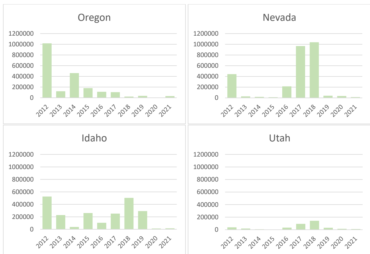
Fig. 3. Declining trends in acres of sage-grouse habitat burned in Oregon between 2012 and 2019 compared to generally increasing trends in nearby states.
