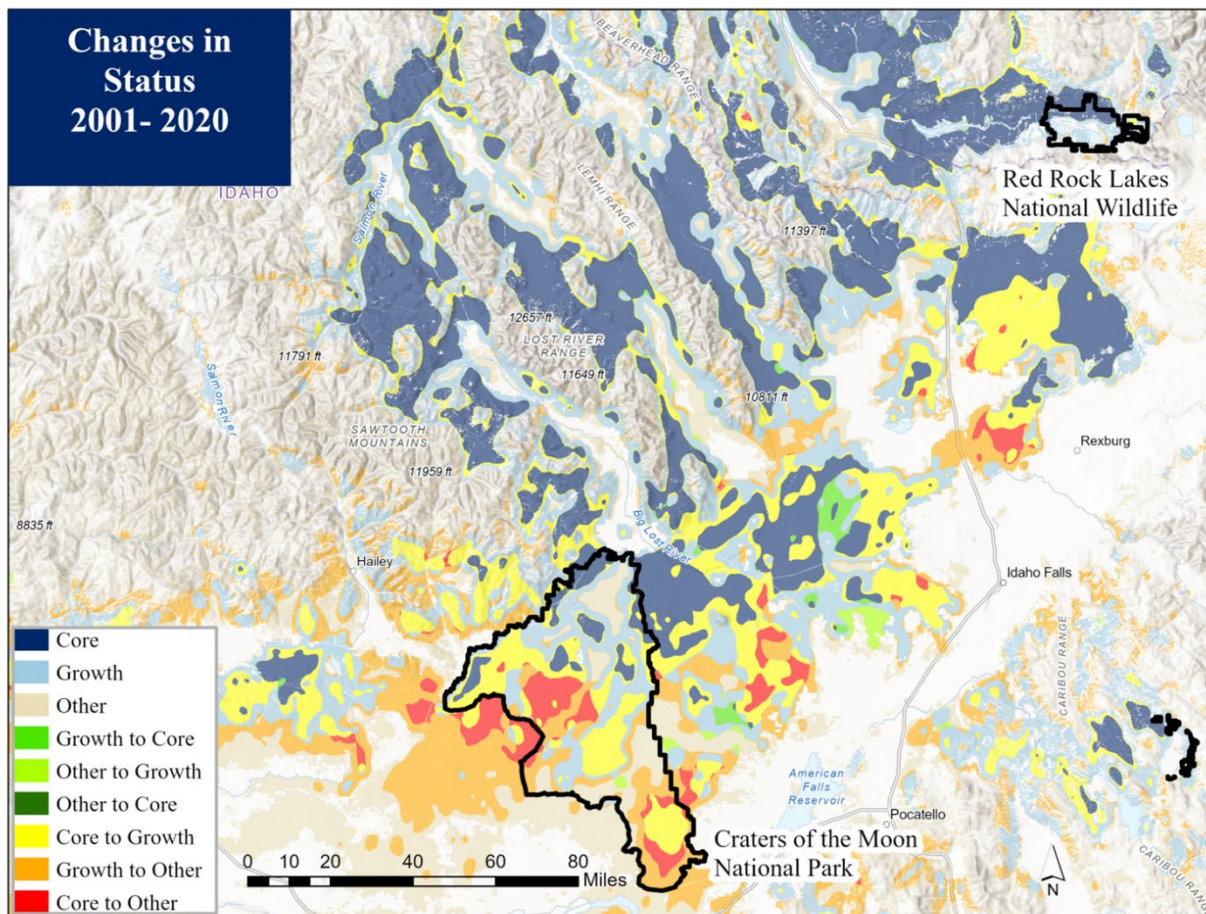
Fig. A3. Evaluating and mapping changes in core, growth, and other rangeland areas over time within areas of interest and regionally can provide context important to defining priority areas as well as indicating which areas are recovering (Growth to Core, Other to Core or Growth) and which are losing ecological integrity (Core to growth or Other, Growth to Other).
